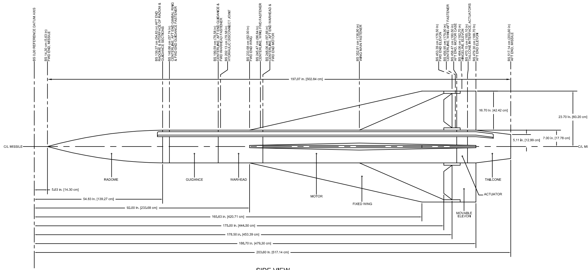
SIDE VIEW
