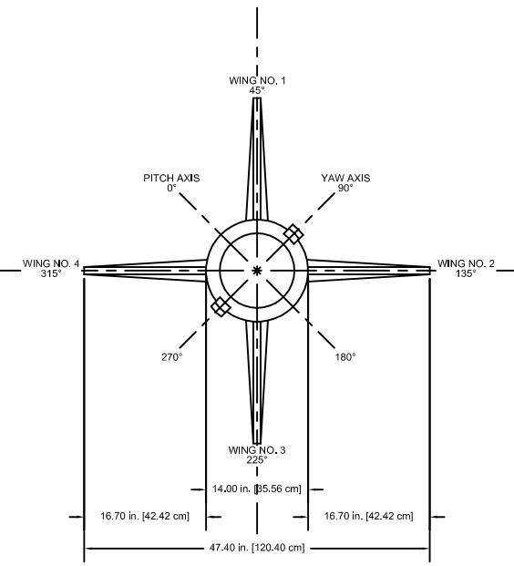
AFT VIEW
